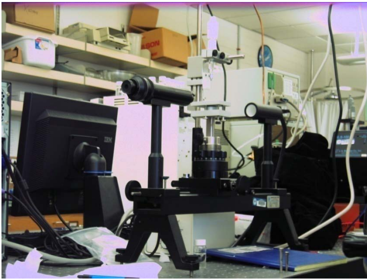
Figure 1.10. Schematic of the contact angle measurement and a photograph of the Ramé-Hart 100 water contact angle goniometer at BYU. A liquid droplet rests on a solid surface. The contact angle, \theta , is the angle between the tangent line of the drop and the solid surface.
