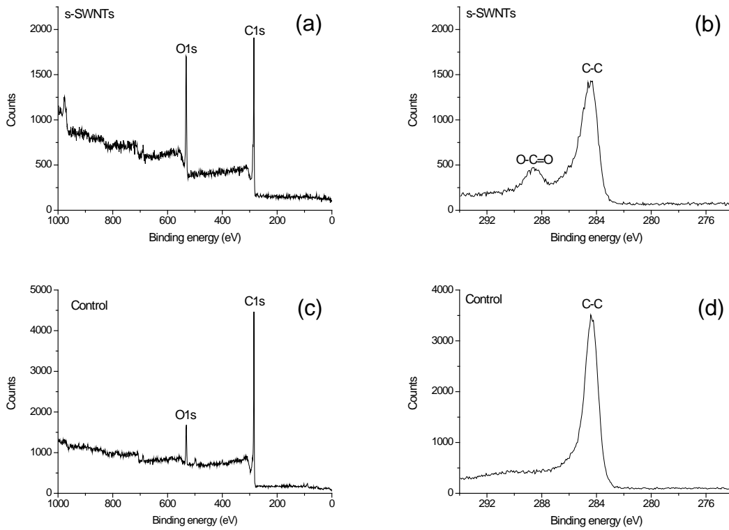
Figure 6.3. XPS survey and carbon 1s narrow scans for an s-SWNTs sample (a and b), and a control sample (c and d). For the control, all reaction conditions were identical to the sample run, with the exception that no peroxide was added.
