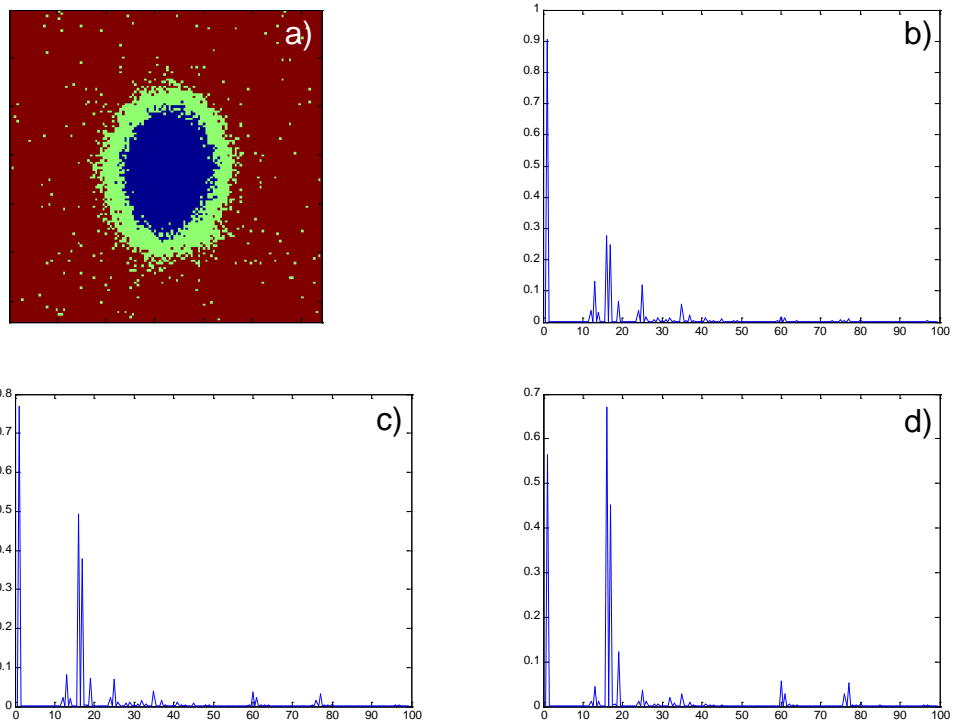
Figure 4.11. (a) Image of the three-cluster analysis of the data shown in Figures 4.7 and 4.8, and average spectra corresponding to the (b) blue, (c) green, and (d) red pixels.
