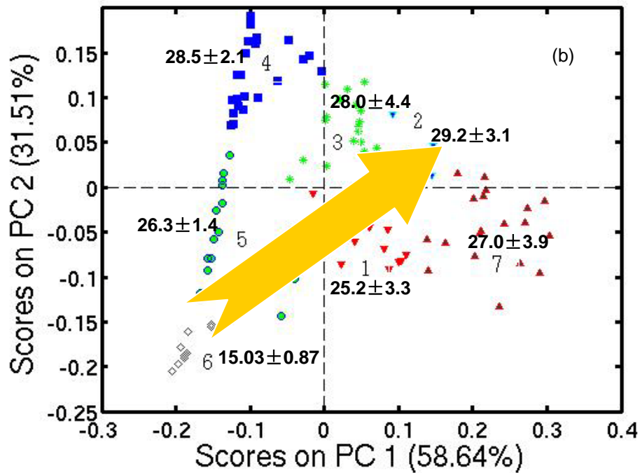
Figure 5.8. (a) PC1 vs. PC2 plot showing the average heating value of the samples found in each of the seven clusters in the dendrogram, and (b) PC1 vs. PC2 plot showing the average percent \text{Al}_2\text{O}_3 composition of the samples found in each of the seven clusters in the dendrogram. The yellow arrows are guides to the eye.
