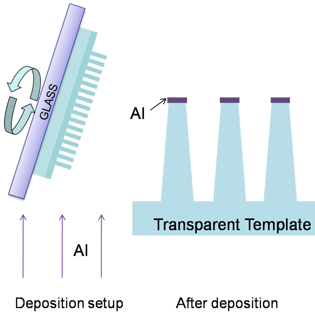
Figure A1.1. Angled thermal evaporation setup for aluminum deposition on a patterned substrate.
